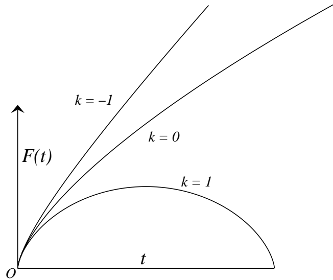
Fig. 5. The Robertson-Walker universe for k = 1 , k = 0 , and k = -1 .
