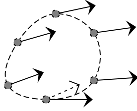
Fig. 3. Paralel displacement along a closed curve in a curved space.
